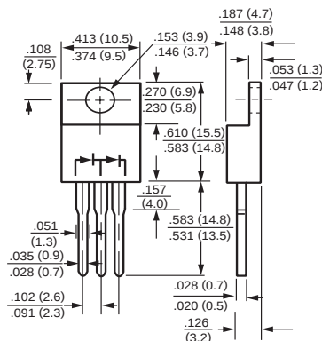
TO-220
