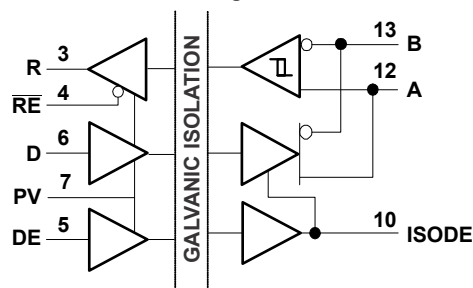
Simplified Schematic
