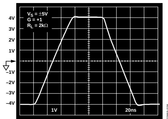
Figure 28. Large Signal Step Response; V_S = \pm 5V , G = +1
