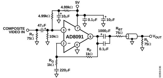
Figure 36. Single-Supply Composite Video Line Driver
