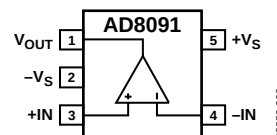
Figure 2. SOT23-5 (RT-5)
