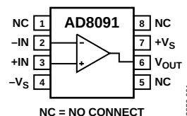
Figure 1. SOIC-8 (R-8)
