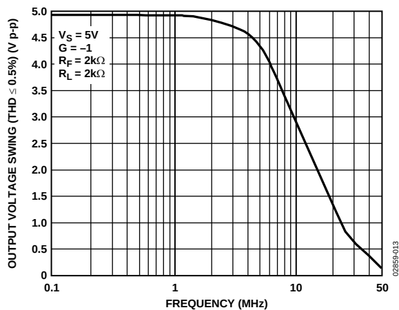
Figure 13. Low Distortion Rail-to-Rail Output Swing
