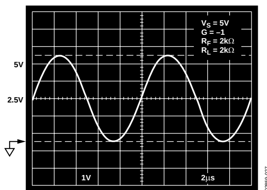
Figure 27. Output Swing; G = -1 , R_L = 2k\Omega
