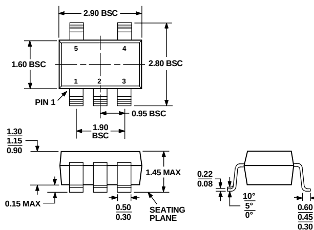
Figure 39. 5-Lead Small Outline Transistor Package [SOT-23] (RT-5)
