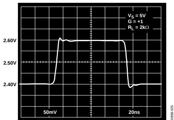
Figure 25. 200 mV Step Response; V_S = +5V , G = +1
