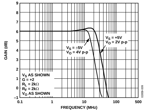
Figure 9. Large Signal Frequency Response; G = +2
