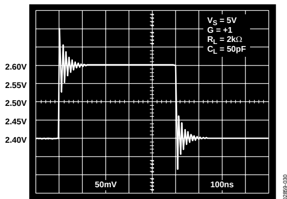
Figure 30. 200 mV Step Response: C_L = 50 \text{ pF}
