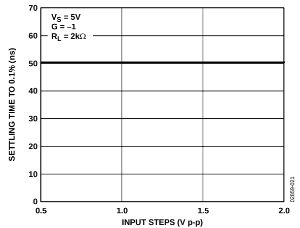
Figure 21. Settling Time vs. Input Step
