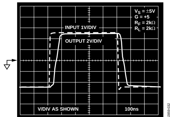
Figure 32. Overdrive Recovery
