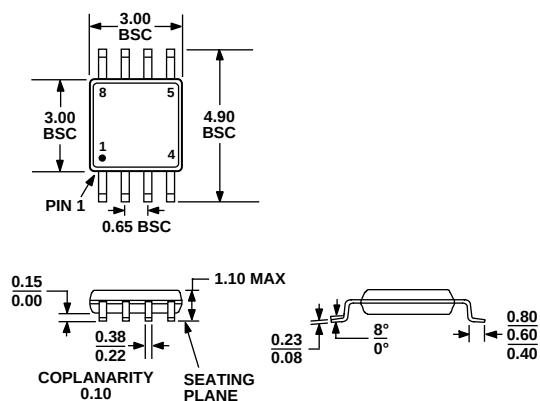
Figure 38. 8-Lead Mini Small Outline Package [MSOP] (RM-8)
