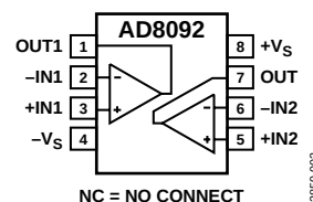
Figure 3. MSOP-8 and SOIC-8 (RM-8, R-8)
