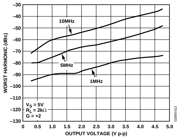
Figure 12. Worst Harmonic vs. Output Voltage
