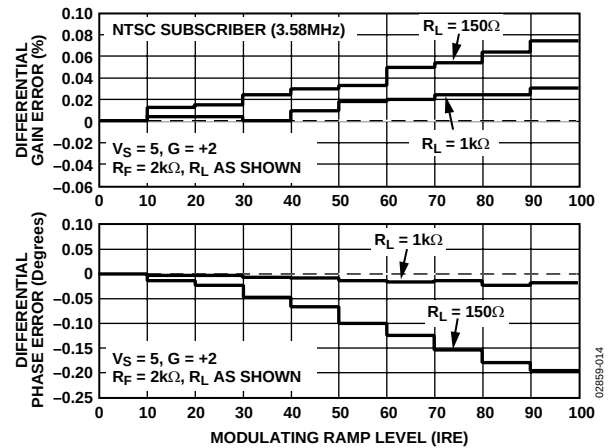
Figure 14. Differential Gain and Phase Errors
