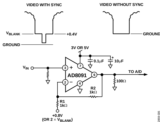
Figure 35. Sync Stripper
