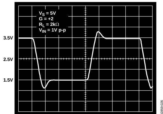
Figure 26. Large Signal Step Response; V_S = +5V , G = +2
