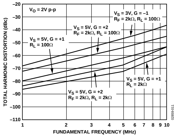
Figure 11. Total Harmonic Distortion
