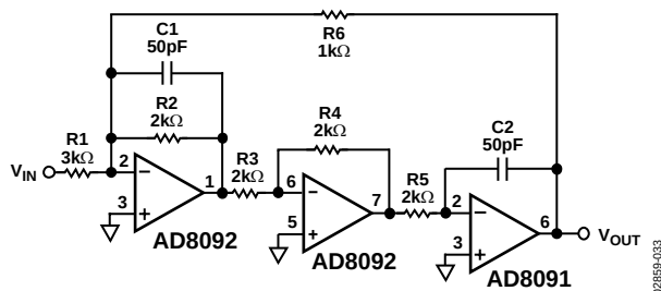
Figure 33. 2 MHz Biquad Band-Pass Filter
