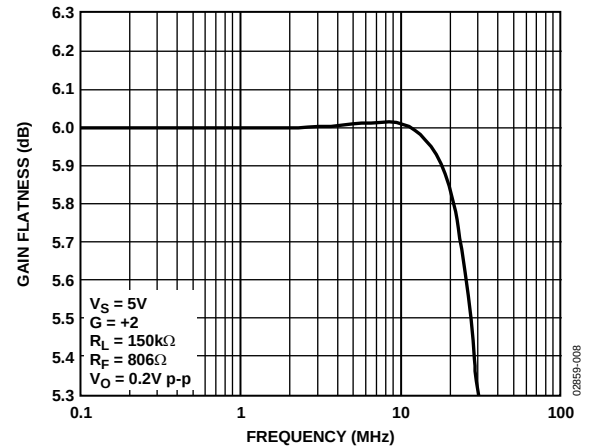
Figure 8. 0.1 dB Gain Flatness vs. Frequency; G = +2
