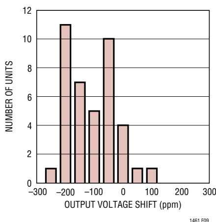
Figure 9. Typical Distribution of Output Voltage Shift After Soldering Onto PC Board
