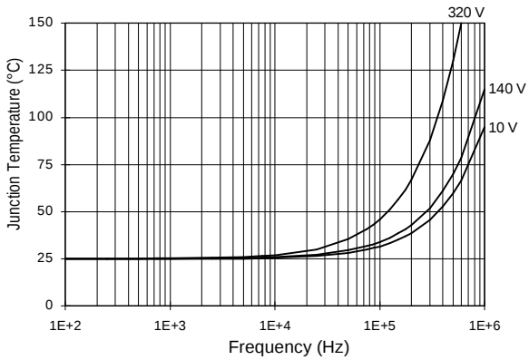
Figure 30. IRS2112 T_j vs. Frequency (IRFBC40) R_{\text{GATE}} = 15 \text{ } \Omega , V_{\text{CC}} = 15 \text{ V}
