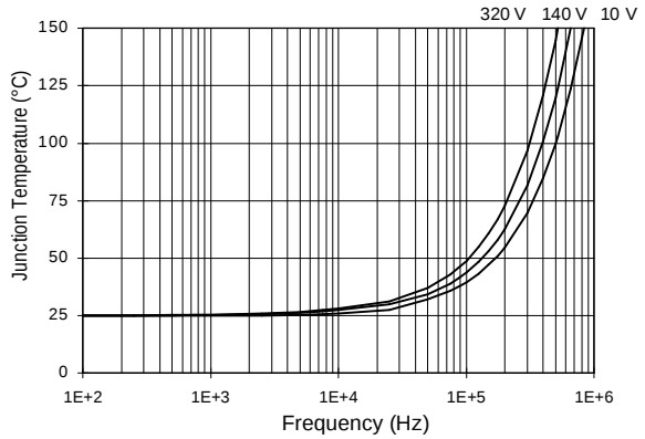
Figure 31. IRS2112 T_j vs. Frequency (IRFPE50) R_{\text{GATE}} = 10 \text{ } \Omega , V_{\text{CC}} = 15 \text{ V}
