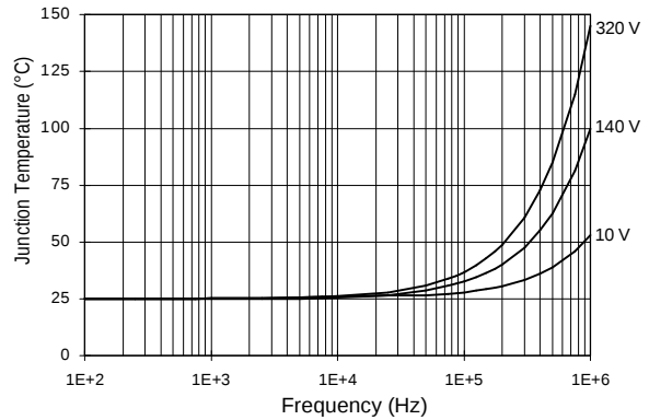
Figure 29. IRS2112 T_j vs. Frequency (IRFBC30) R_{\text{GATE}} = 22 \text{ } \Omega , V_{\text{CC}} = 15 \text{ V}
