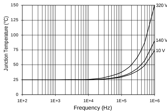
Figure 32. IRS2112S T_j vs. Frequency (IRFBC20) R_{\text{GATE}} = 33 \text{ } \Omega , V_{\text{CC}} = 15 \text{ V}
