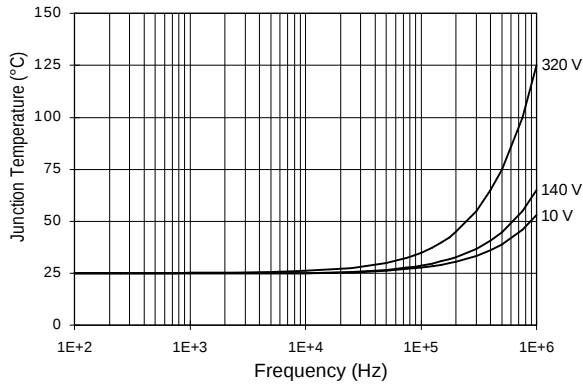
Figure 28. IRS2112 T_j vs. Frequency (IRFBC20) R_{\text{GATE}} = 33 \text{ } \Omega , V_{\text{CC}} = 15 \text{ V}
