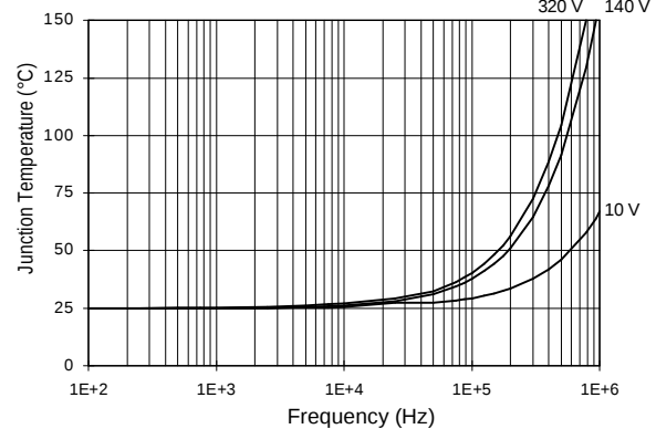
Figure 33. IRS2112S T_j vs. Frequency (IRFBC30) R_{\text{GATE}} = 22 \text{ } \Omega , V_{\text{CC}} = 15 \text{ V}
