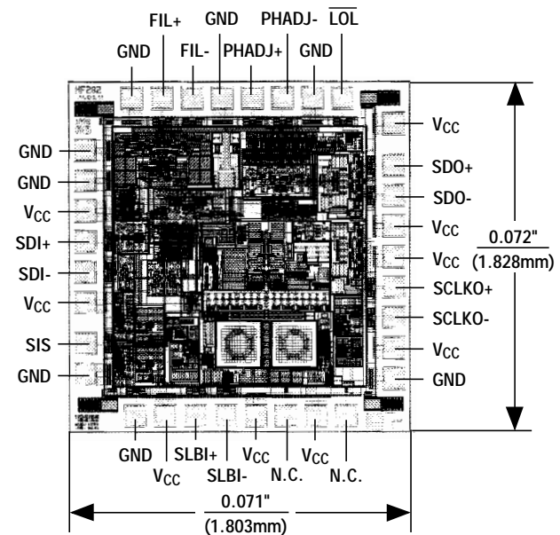
Chip Topography
