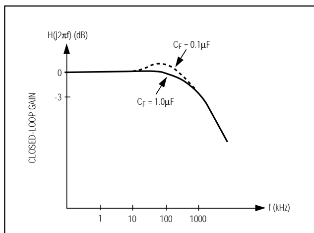
Figure 5. Closed-Loop Transfer Function
