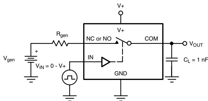
Figure 4. Charge Injection
