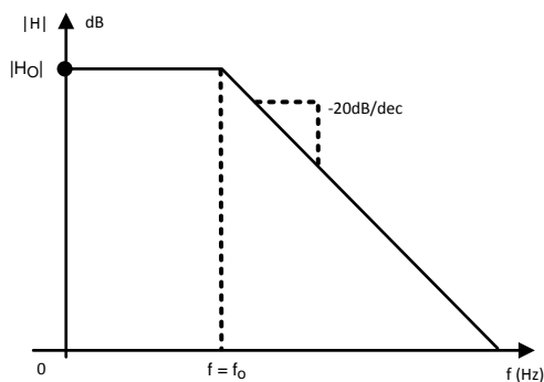
Figure 8. Lowpass Filter Transfer Function
