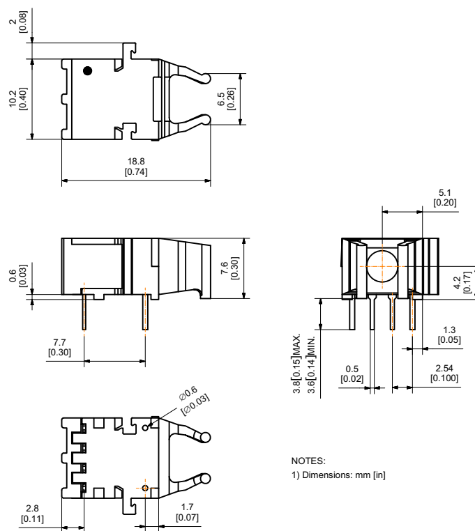
Figure 2 Mechanical Dimensions - Horizontal Packages
