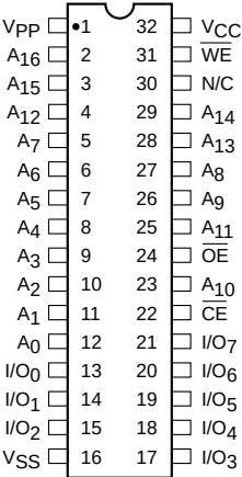
DIP Package (L)
