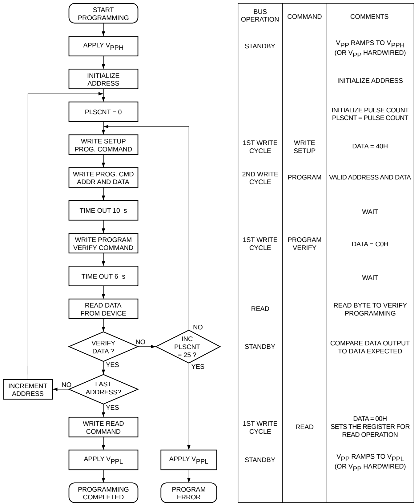
Figure 7. Programming Algorithm(1)
