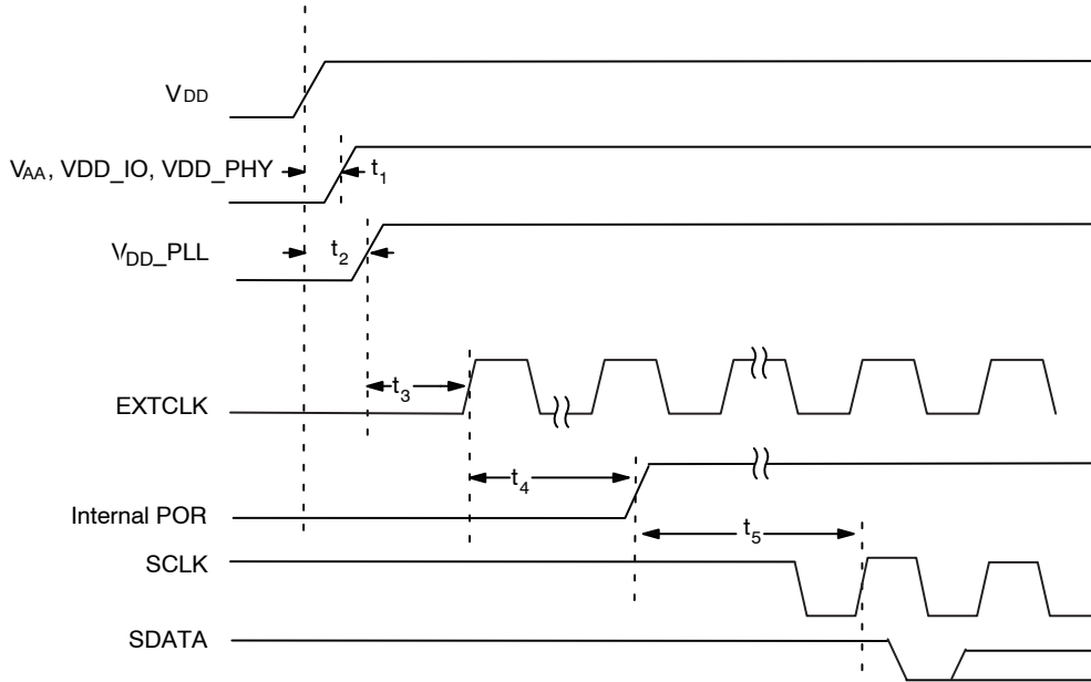
Figure 34. Power-Up Sequence
