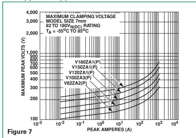
V82ZA2(P) - V180ZA1(P)
