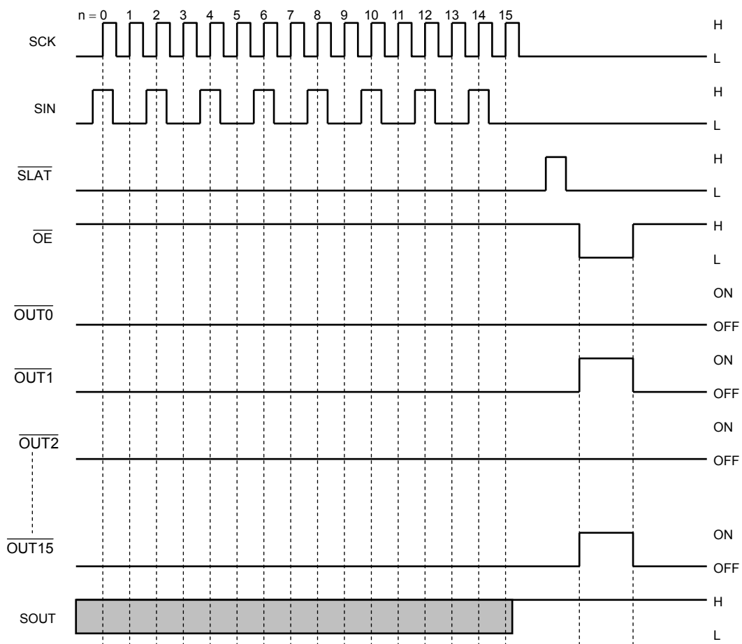
Timing Diagram
