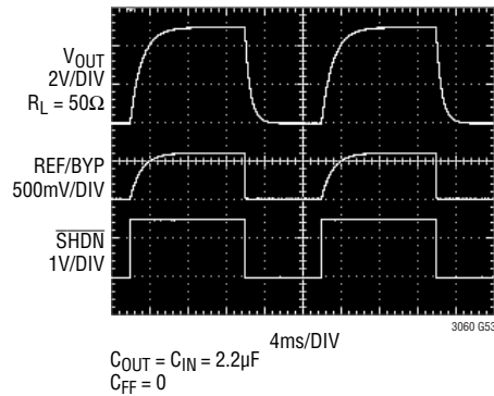
SHDN Transient Response C_{\text{REF/BYP}} = 10\text{nF}
