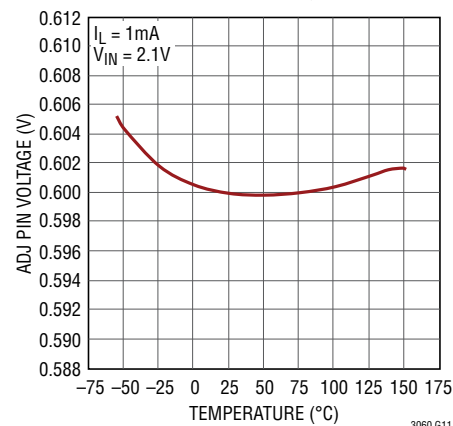
LT3060 ADJ Pin Voltage
