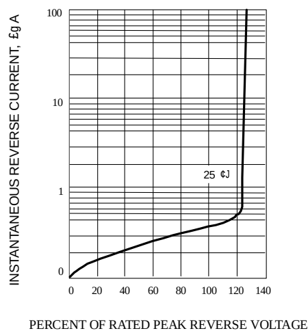
Fig. 4-REVERSE CHARACTERISTICS
