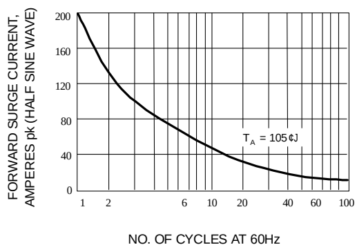
Fig. 1-NON-RECURRENT SURGE RATING
