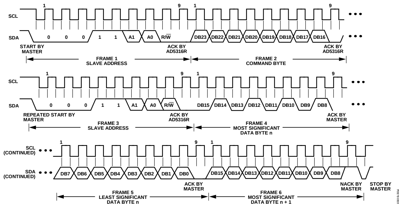
Figure 43. I²C Read Operation
