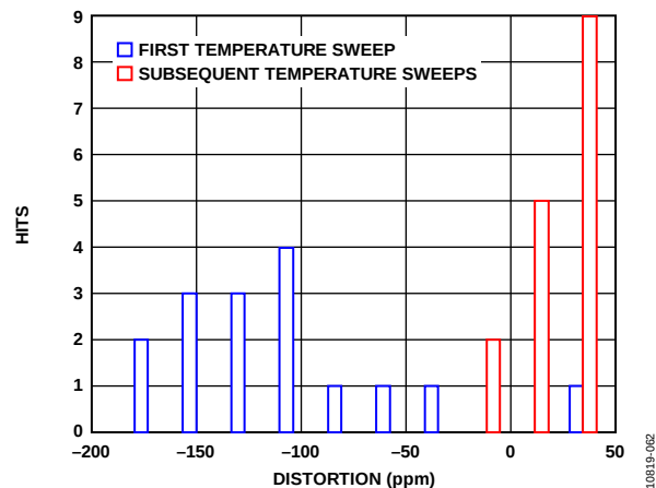
Figure 48. Thermal Hysteresis
