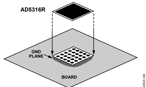
Figure 50. Paddle Connection to Board
