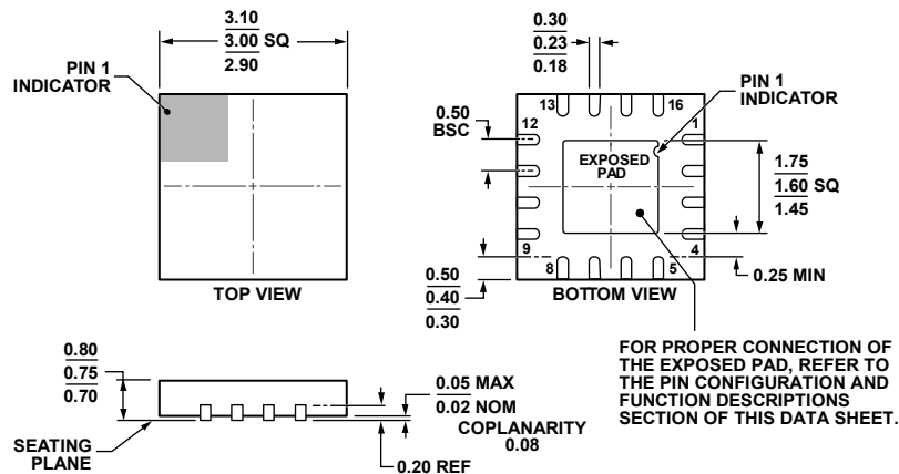
Figure 52. 16-Lead Lead Frame Chip Scale Package [LFCSP_WQ] 3 mm × 3 mm Body, Very Very Thin Quad (CP-16-22) Dimensions shown in millimeters
