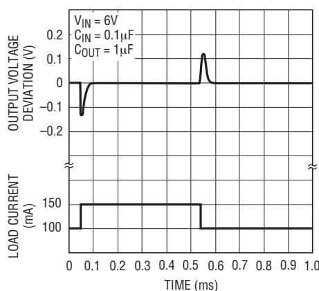
LT1121-5 Load Transient Response
