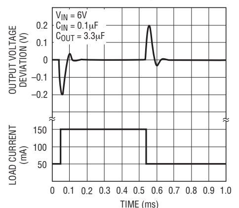
LT1121-5 Load Transient Response
