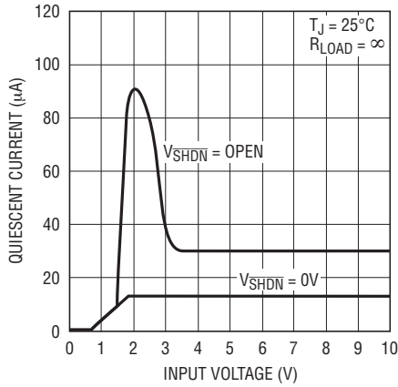
LT1121-3.3 Quiescent Current
