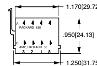
VCH CONNECTOR HOUSING
