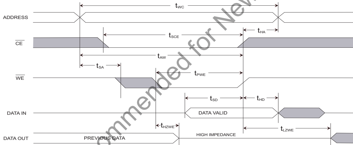
Figure 10. SRAM Write Cycle 2: \overline{CE} Controlled [13, 14]
