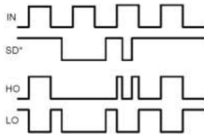
Figure 1. Input / Output Timing Diagram
