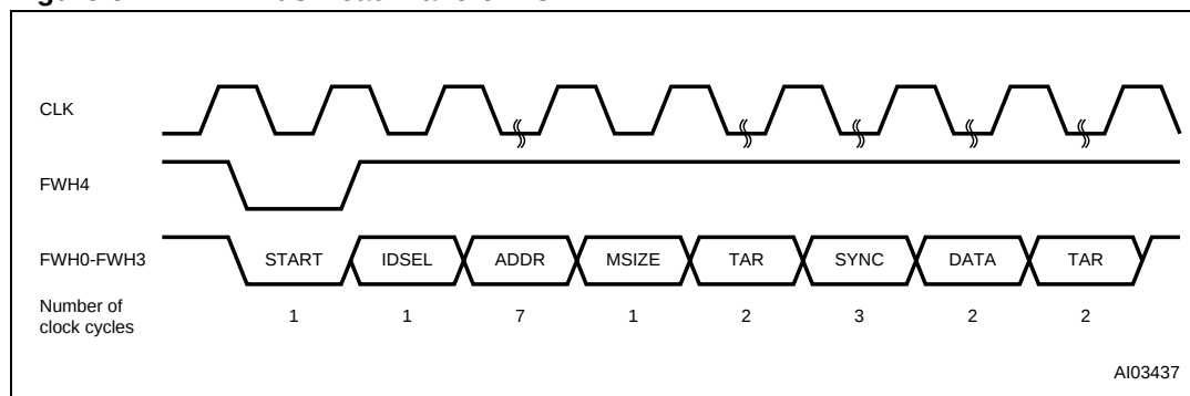
Figure 6. FWH Bus Read waveforms
