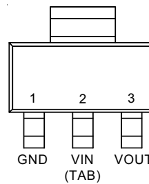
SOT-223 (L-Type)
