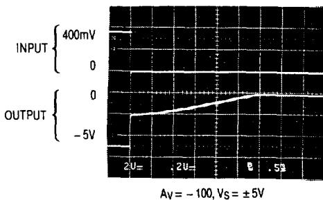
Overload Recovery
