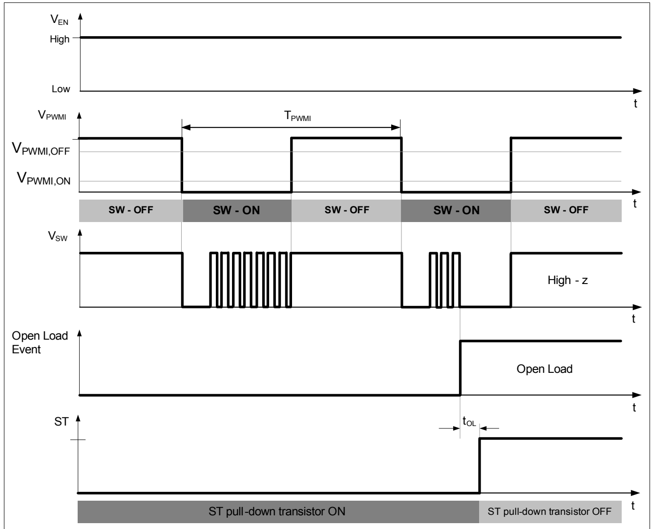
Figure 9 Open Load diagnosis via \mu C connected to ST pin
