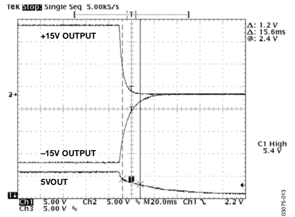
Figure 13. +15 V and -15 V Outputs at Power-Down
