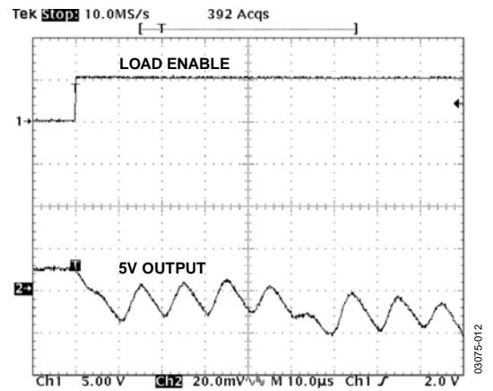
Figure 12. Output Transient Response for Maximum Load Current
