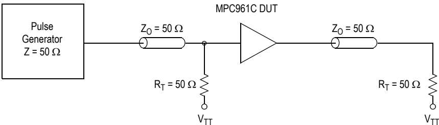
Figure 11. TCLK MPC961C AC Test Reference for V_{CC} = 3.3\text{ V} and V_{CC} = 2.5\text{ V}
