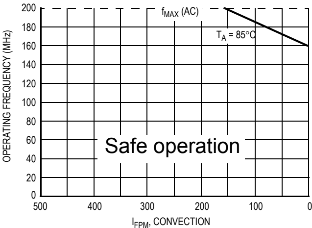
Figure 9. Maximum MPC961C Frequency, V_{CC} = 3.3\text{ V} , MTBF 9.1 Years, Driving Series Terminated Transmission Lines
