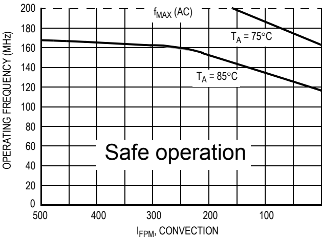
Figure 10. Maximum MPC961C Frequency, V_{CC} = 3.3\text{ V} , MTBF 9.1 Years, 4 pF Load per Line
