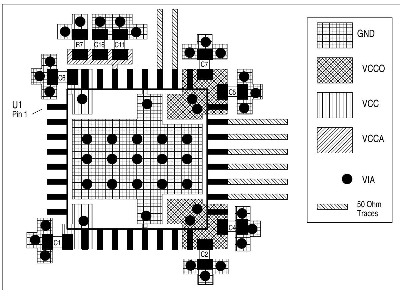
FIGURE 5B. PCB BOARD LAYOUT FOR ICS8735I-01
