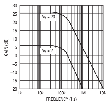
Programmable Gain Amplifier Frequency Response
