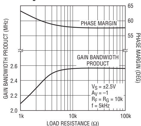
Gain Bandwidth and Phase Margin vs Load Resistance
