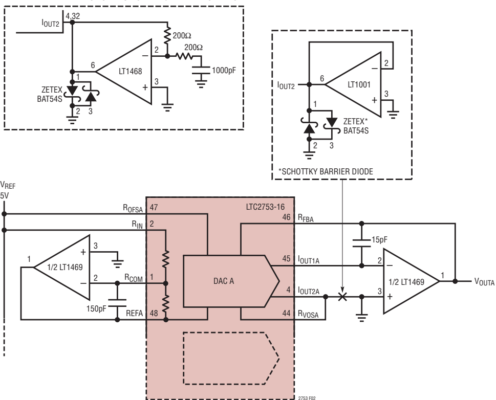
ALTERNATE AMPLIFIER FOR OPTIMUM SETTLING TIME PERFORMANCE
