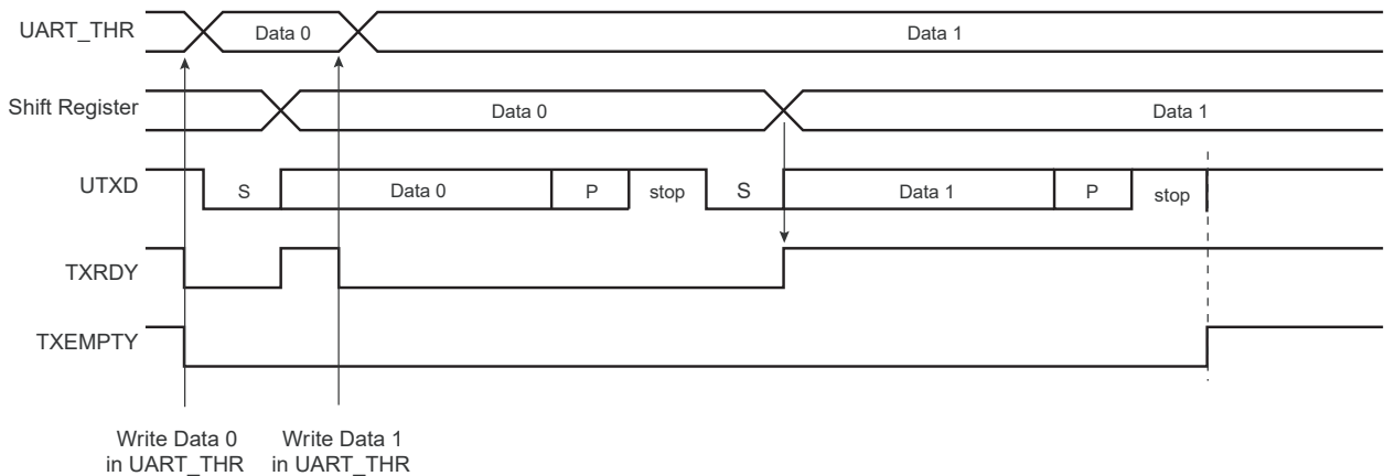
Figure 47-10. Transmitter Control
