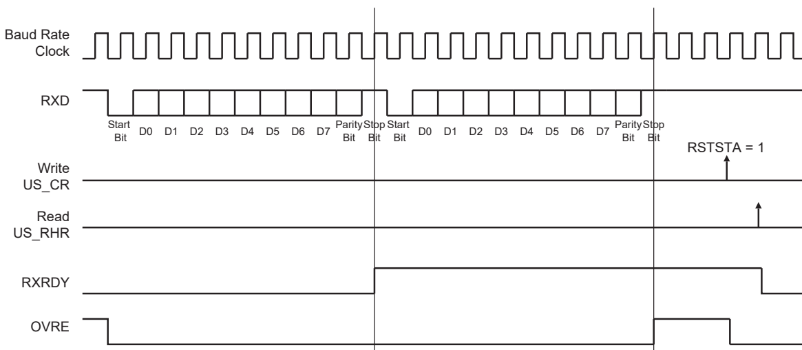
Figure 46-20. Receiver Status
