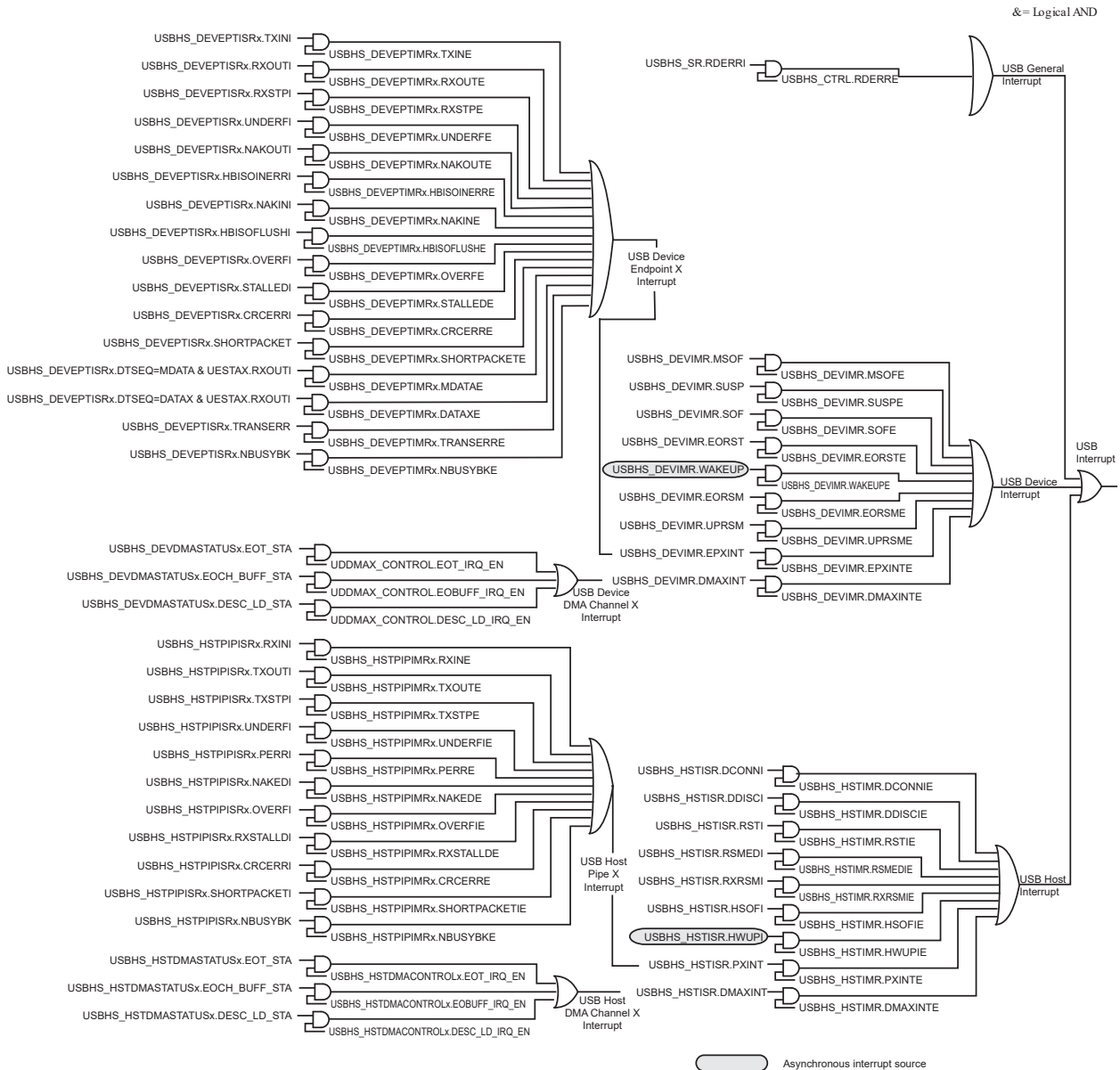
Figure 39-3. Interrupt System
