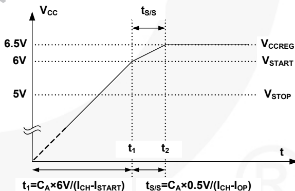
Figure 20. Soft-Start Function
