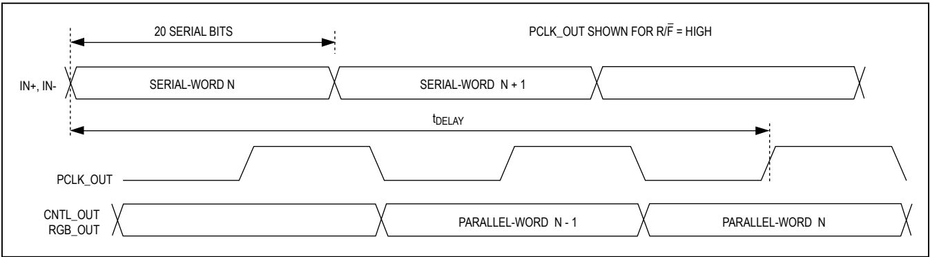
Figure 6. Deserializer Delay
