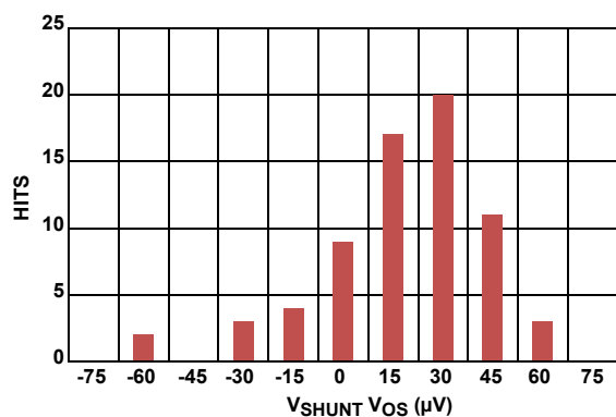
FIGURE 3. V_{SHUNT} V_{OS}
