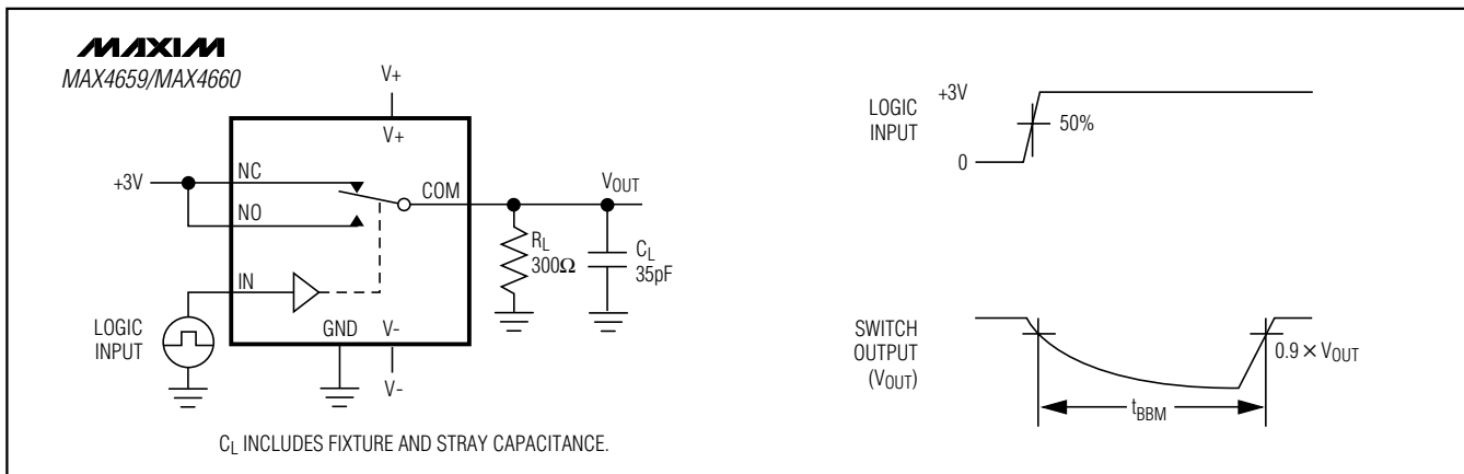
Figure 3. Break-Before-Make Time
