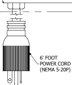
ASSEMBLY - VIEW FROM BOTTOM
