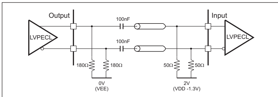
Figure 6. LVPECL output termination, AC-coupled.
