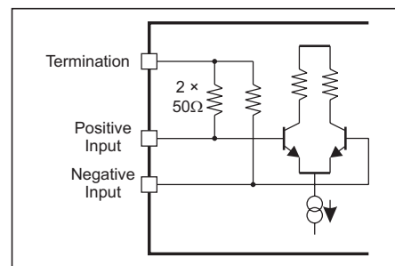
Figure 9. CML input buffer
