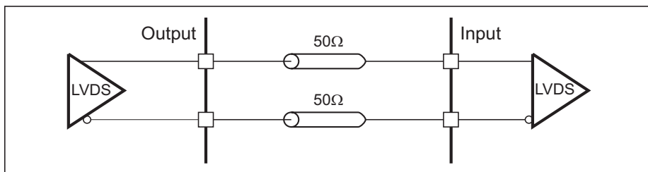
Figure 5. LVDS connection
