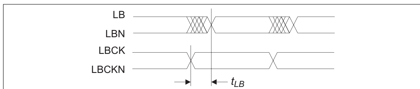
Figure 26. Loop-back Timing.
