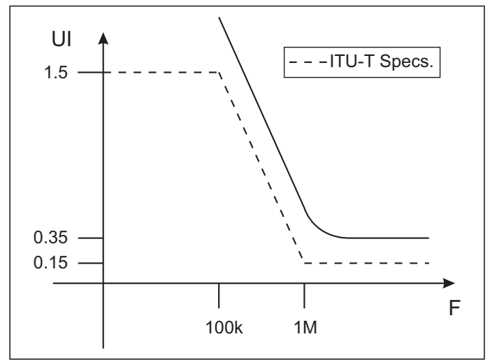
Figure 28. Jitter Tolerance
