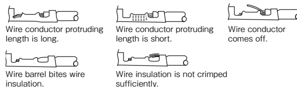
Fig.2: Examples of defective crimping
