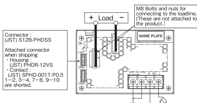
Attached connector when shipping
