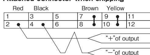
Attached connector when shipping
