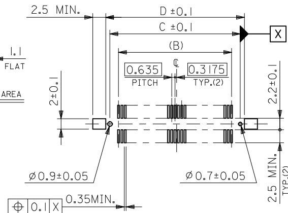
推奨基板寸法 RECOMMENDED PCB PATTERN LAYOUT
