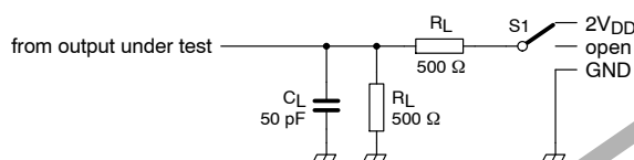
Figure 17. Load Circuit
