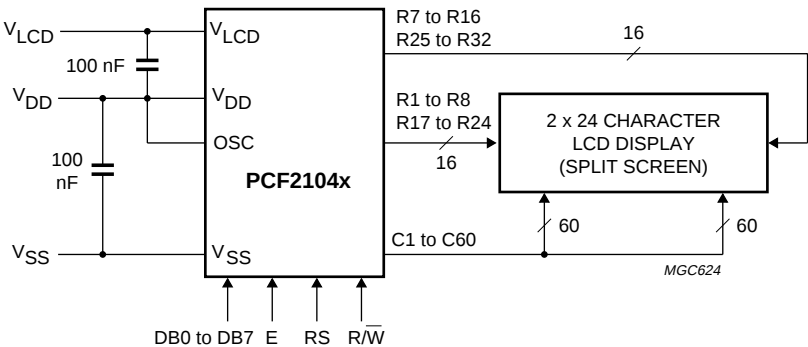
Fig.30 Typical application using parallel interface.
