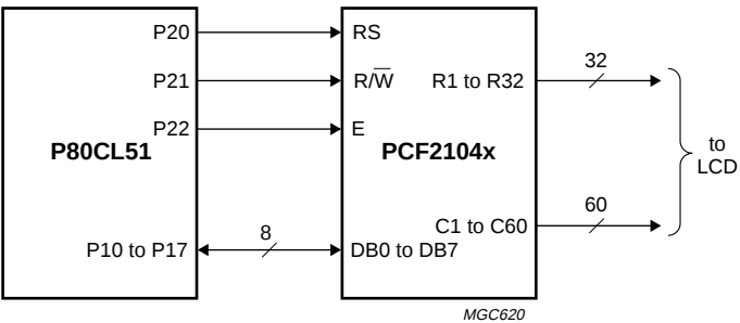
Fig.28 Direct connection to 8-bit microcontroller; 8-bit bus.
