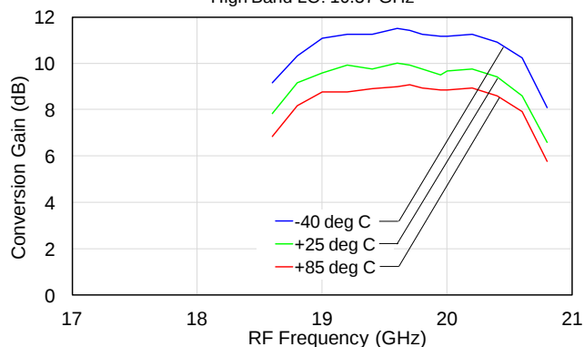
CG vs. Frequency vs. Temperature High Band LO: 10.57 GHz
