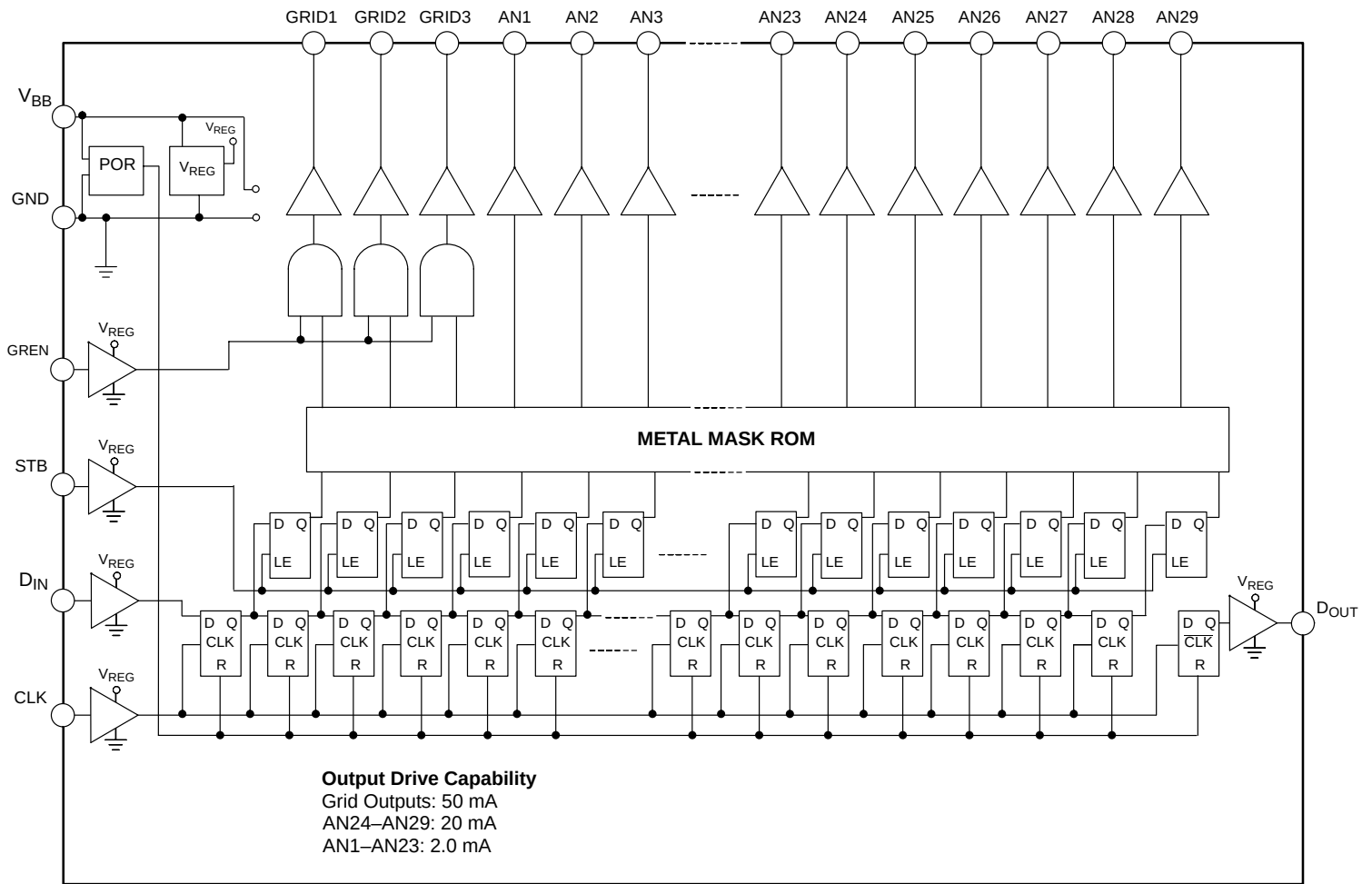
Figure 2. Block Diagram
