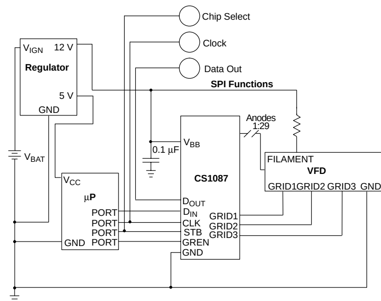
Figure 1. Application Diagram
