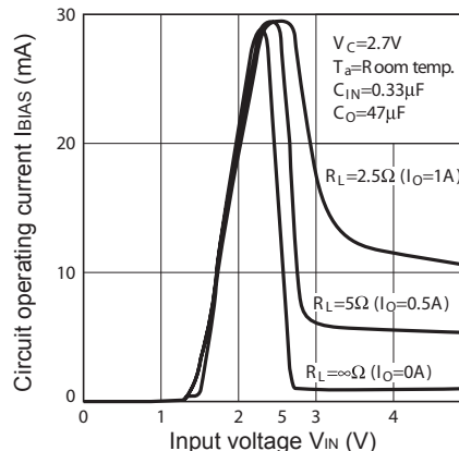
Fig.36 Circuit Operating Current vs. Input Voltage (PQ025EZ01ZxH)
