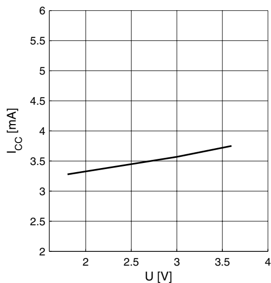
Supply Current I_{CC} = f(V)
