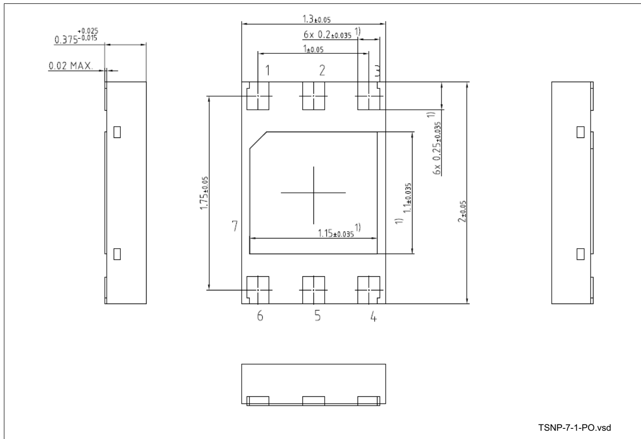
Figure 8 Package Outline (Top, Side and Bottom View)
