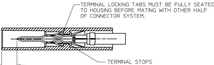
SECTION "B"- "B" NO SCALE
