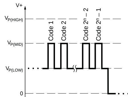
Figure 5. Bit field addressing pulse train. Addressing the bit field by incrementing the code causes the programmable parameter value to change. The number of bits available for a given programming code, n , varies among parameters; for example, the bit field for V_{OUT(Q)} has 6 bits available, which allows 63 separate codes to be used.
