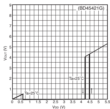
I/O characteristic
