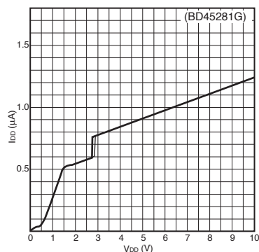
Circuit current
