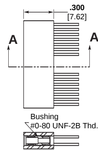
Section A-A Plug
