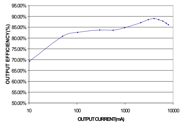
Fig. 16 Output efficiency
