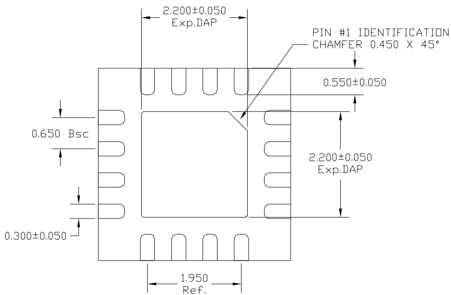
BOTTOM VIEW
