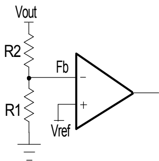
Figure 17 - Voltage Divider
