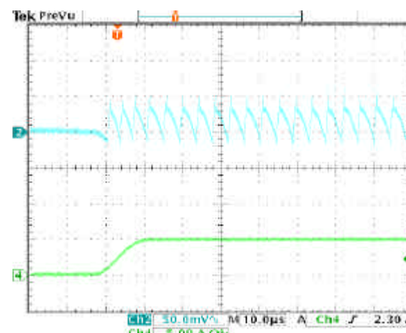
Fig. 14 Dynamic response in PFM mode (CH2 1.8V OUTPUT AC, CH4 OUTPUT CURRENT)
