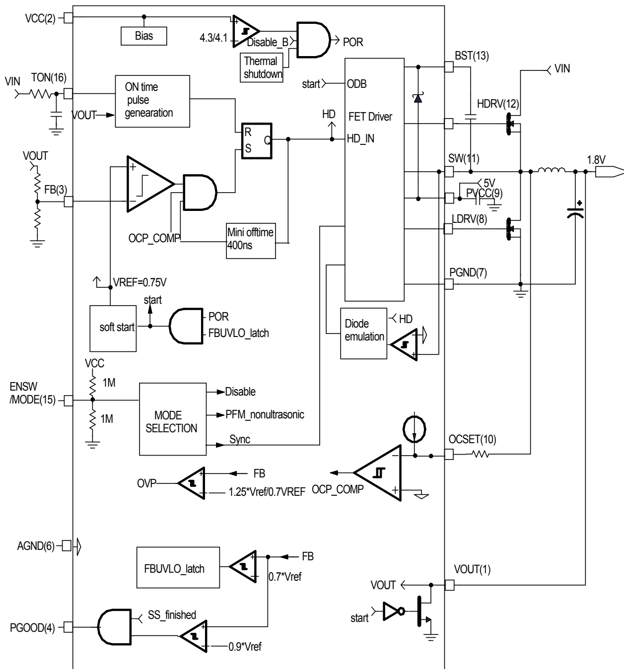
Figure 2 - Simplified block diagram of the NX2138
