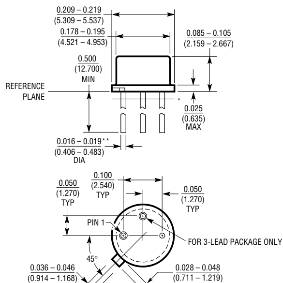
H Package 2-Lead and 3-Lead TO-46 Metal Can (LTC DWG # 05-08-1340)
